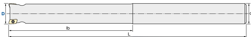
Fig. 2: Carbide Shank
