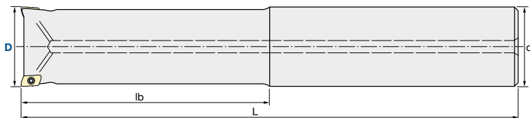
Fig. 1: Steel Shank
